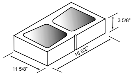
12" Scored Brick
